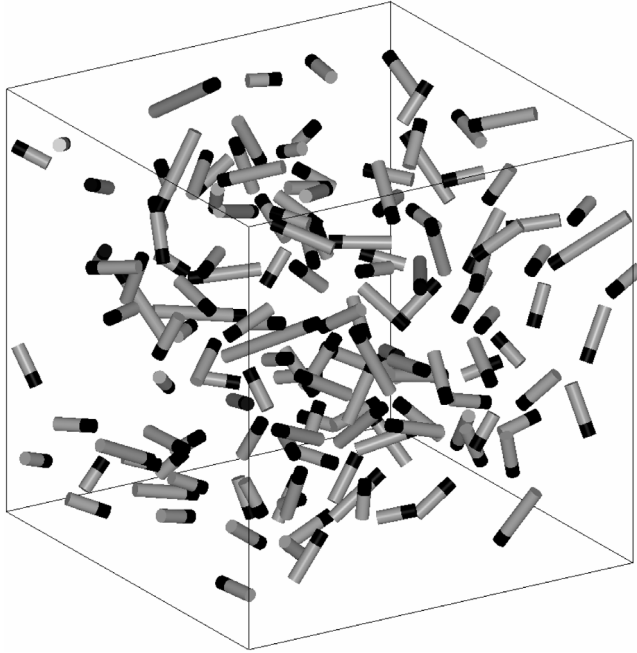
FIGURE 9. Velocities of squirmers c=0.4 ( \beta=5 and G_{bh}=0 ). Only the velocities larger than 1 are shown as cylinders, in which the length of a cylinder is the absolute value of the velocity, and the centre position of the corresponding squirmer is expressed by a black tip. In some regions, neighbouring squirmers are swimming in similar directions.
