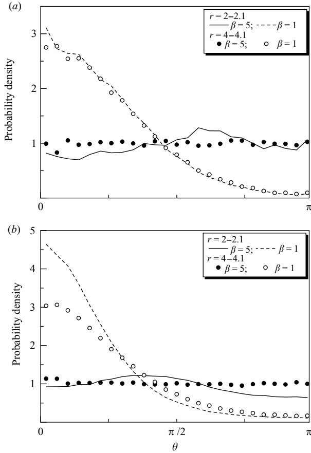
FIGURE 14. The probability density of two squirmers having an angle \theta between their orientation vectors and whose distance apart is between either 2 and 2.1 or 4 and 4.1 for different values of c and \beta (averaged between t=500-1500 with N=64 ). (a) c=0.1 ; (b) c=0.4 .
