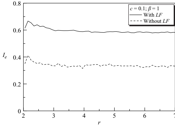
FIGURE 20. The effect of lubrication forces on the spatial correlation of the orientation of the squirmers ( c=0.1 , \beta=1 and N=64 ). The coefficients for the lubrication force are \alpha_1=1 and \alpha_2=20 . The inclusion of the near-field lubrication forces in constructing the grand resistance matrix is indicated by with LF, whereas without LF indicates that they are not included.
